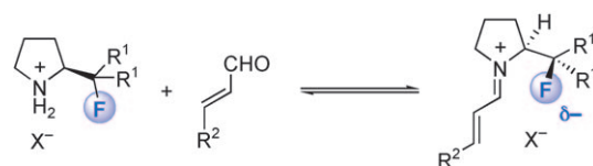
Scheme 1. The fluorine-iminium ion gauche effect.
